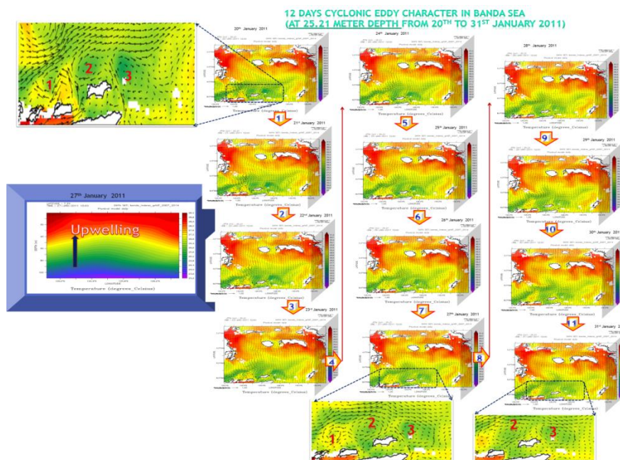
Figure 2. The 12 days unique character of cyclonic Eddies current in Banda sea. The inset with blue color frame shows the significant indicator of upwelling temperature process in the three cyclonic eddies in Banda sea, for example on 27 th January 2011.
