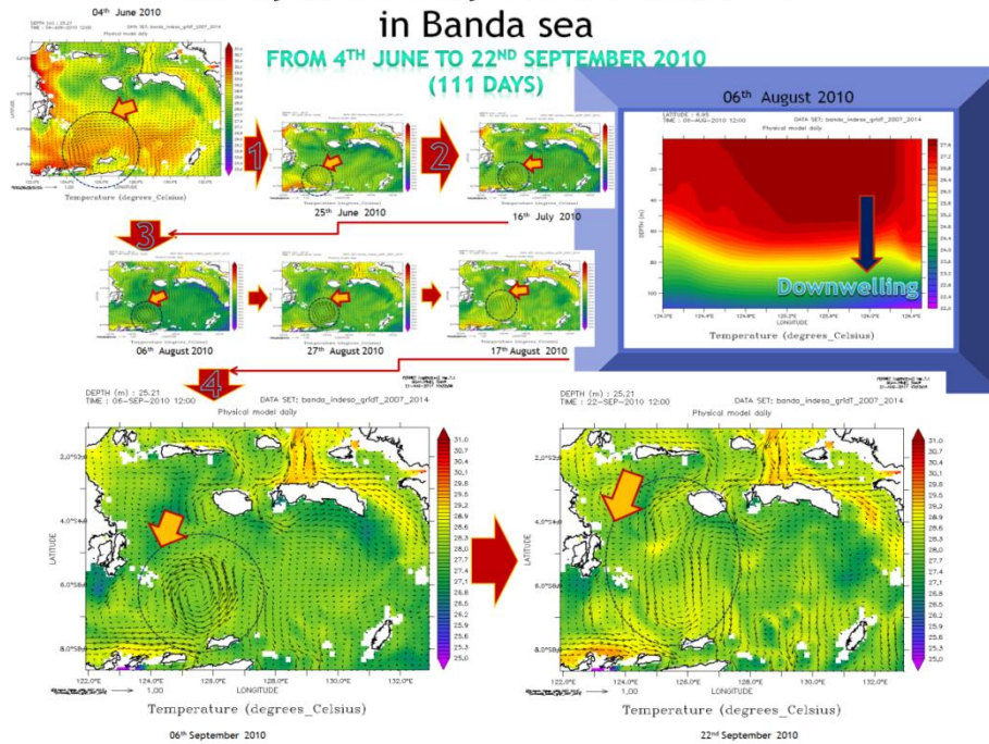
Figure 1. The 111 days unique character of anti-cyclonic Eddy current in Banda sea. The inset explains downwelling temperature behavior of an anti-cyclonic eddy, for example recorded on 6 th August 2010.
